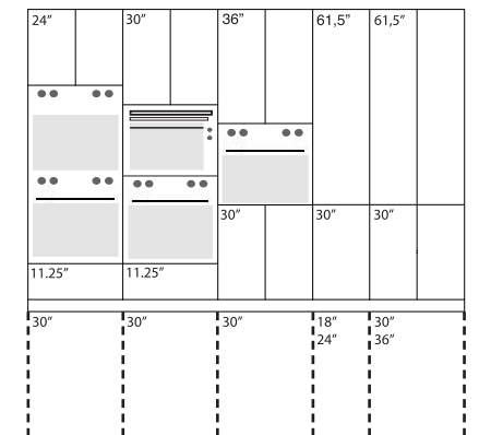
BASE UNITS H 96" D 24" + DOOR
